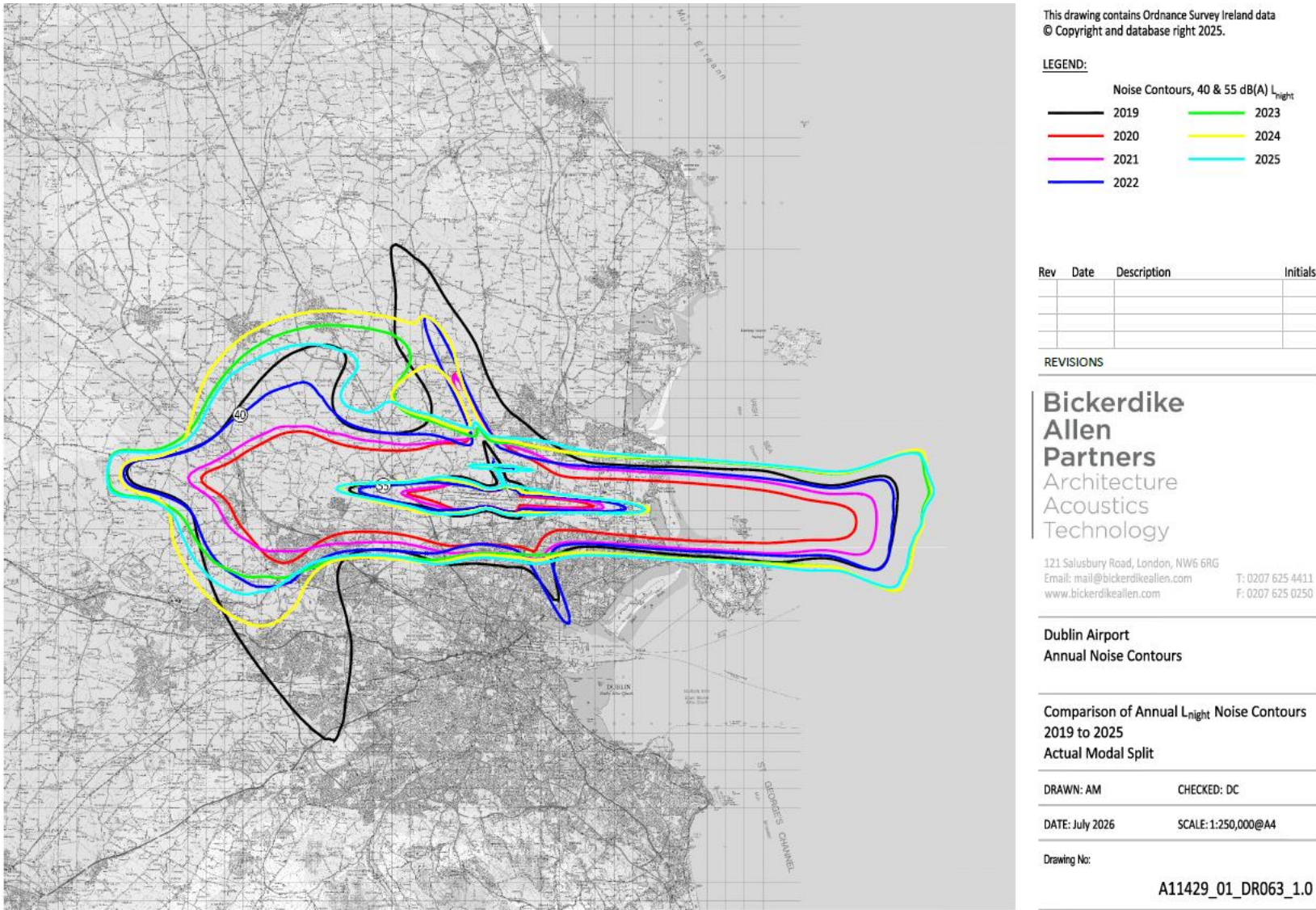
Figure 5.2 - Comparison of Annual Lnight Noise Contours 2019 to 2025
