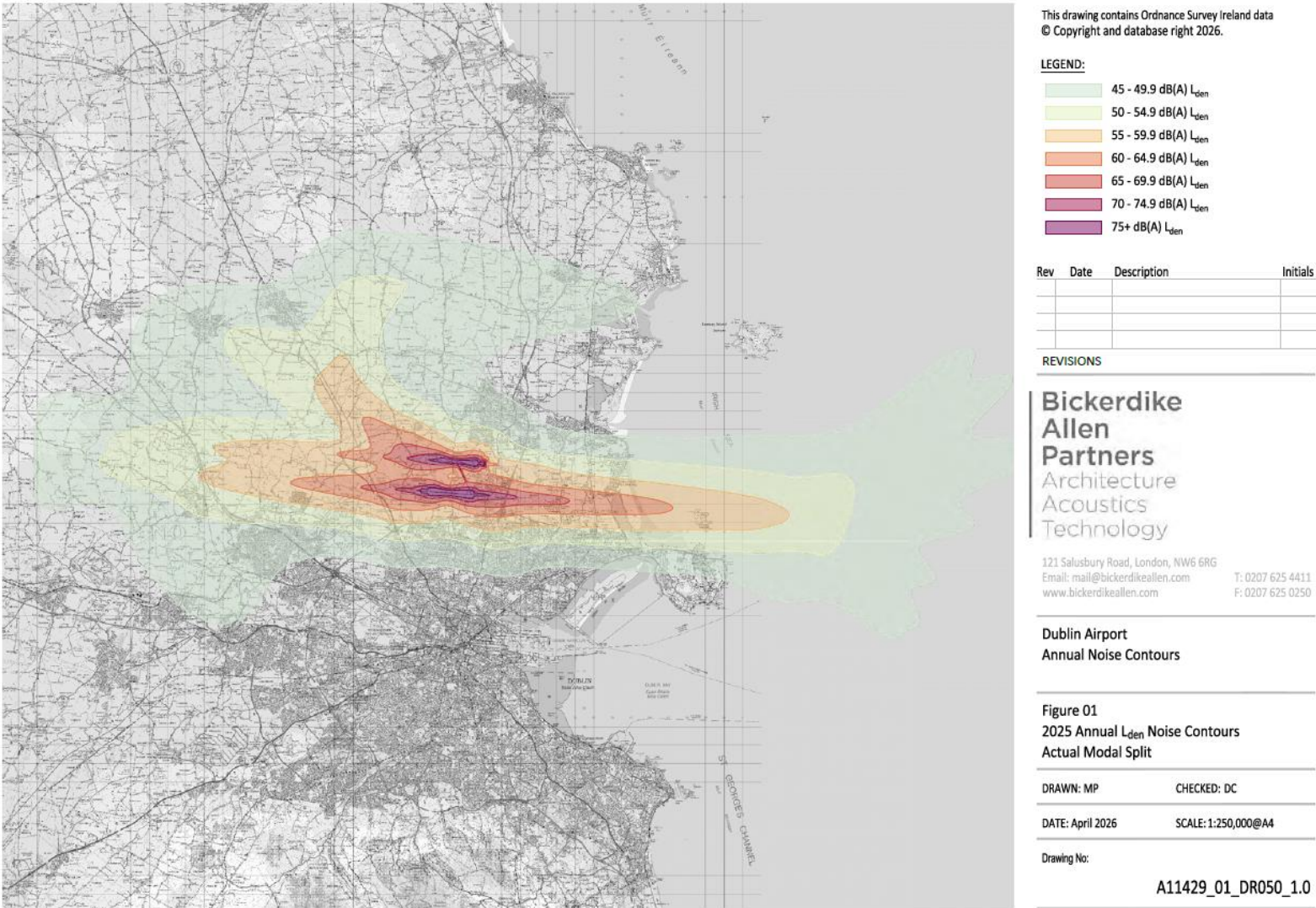
Figure 5.3 - 2025 Annual Lden contours (45 - 75+ dBA)
