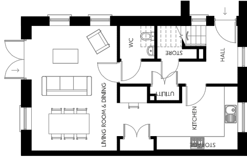
Ground Floor
