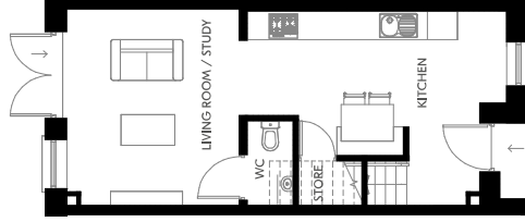
Ground Floor
