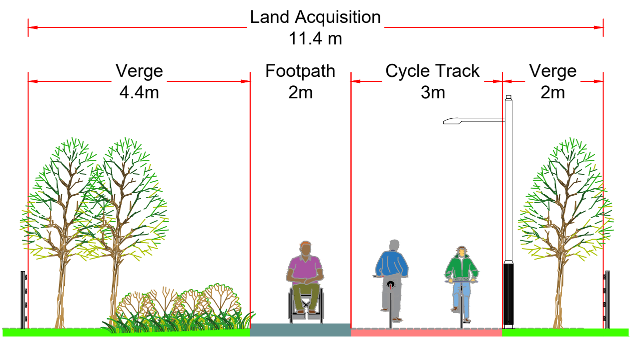
PROPOSED SECTION C-C SCALE - 1:75
