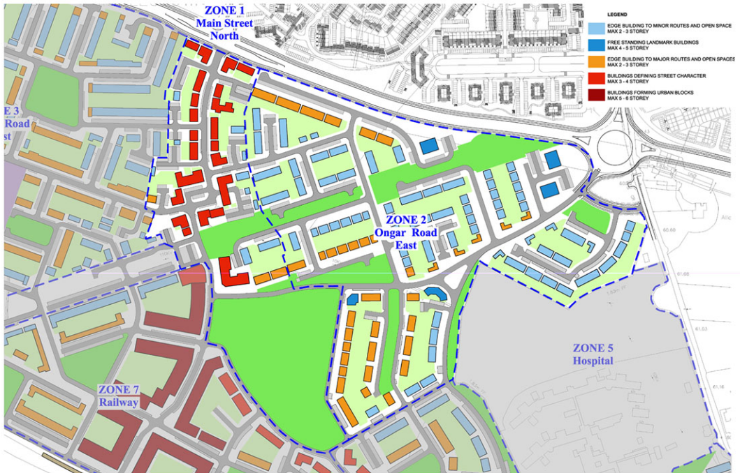
Fig 5.2.1 Indicitive Design Analysis Zones 1 and 2
