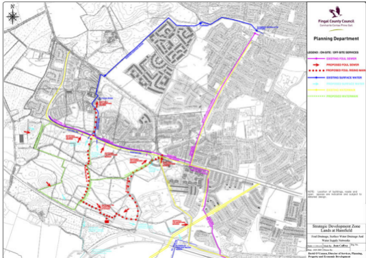
Fig 13.5.7 Service Infrastructure
