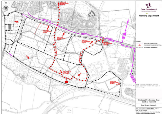
Fig 9.1 Foul Sewer Network
