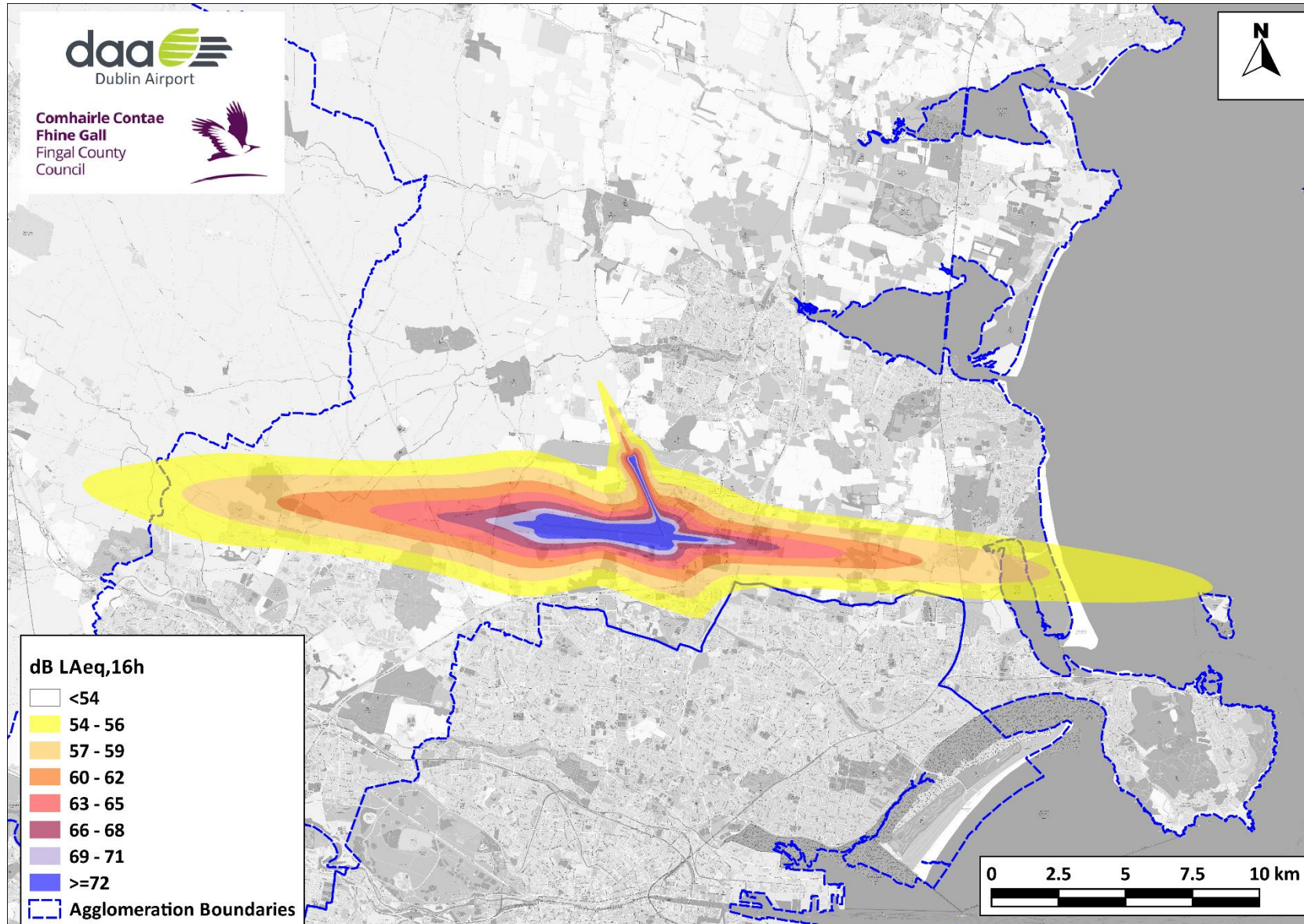
Figure 10 – 2016 L_{Aeq, 16hr} Noise Exposure Contours
